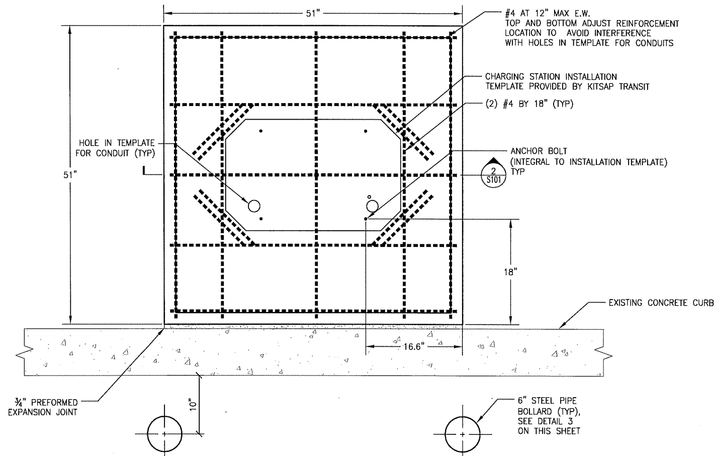
CHARGING STATION FOUNDATION PLAN
