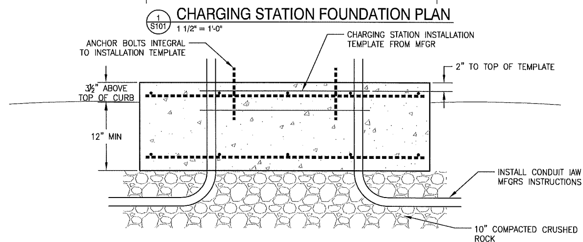
CHARGING STATION FOUNDATION SECTION
