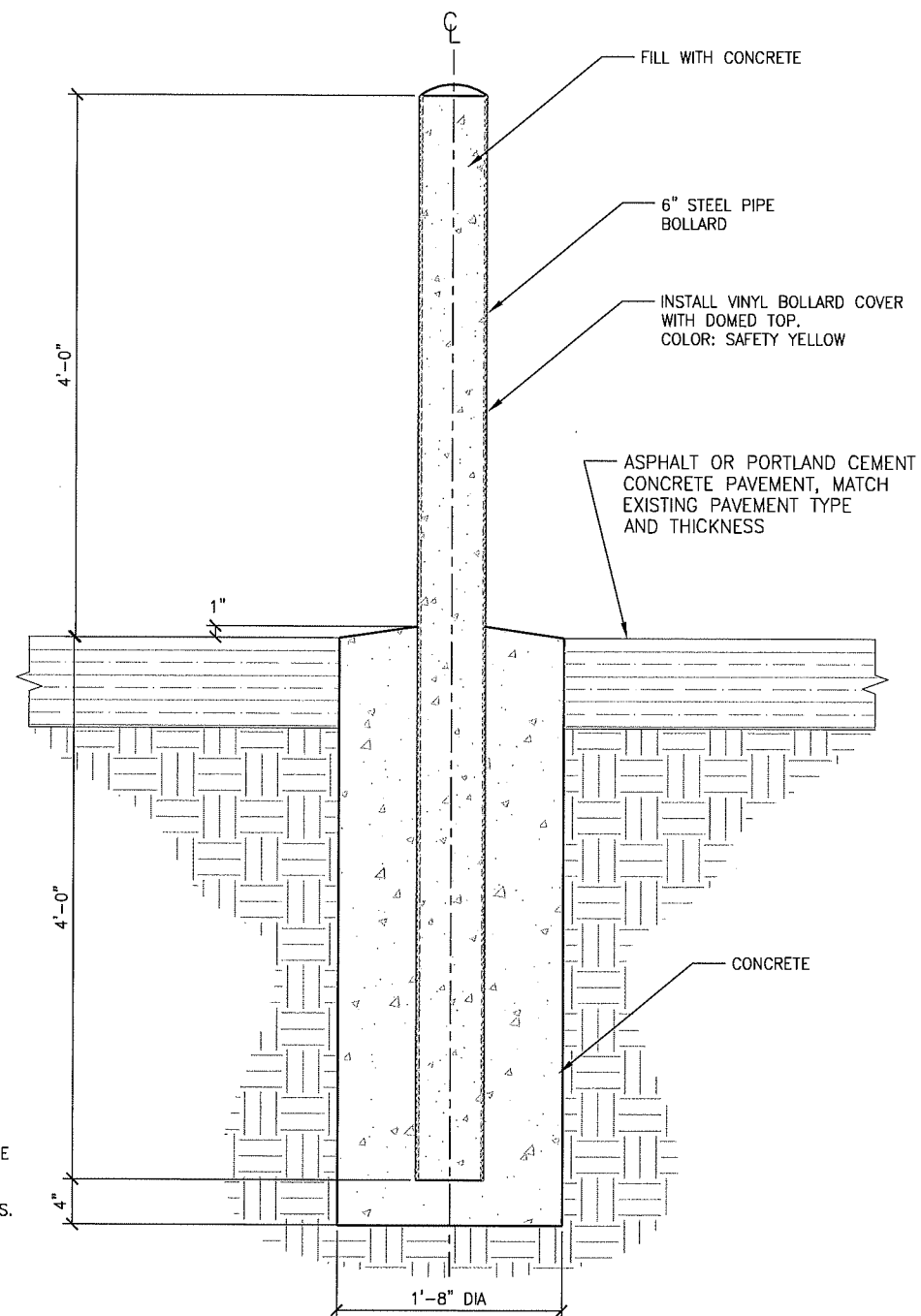
CHARGING STATION BOLLARD DETAIL
